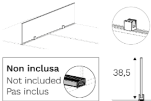
side screens for central profile
